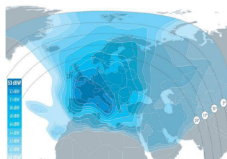
Hotbird @ 13° Est
